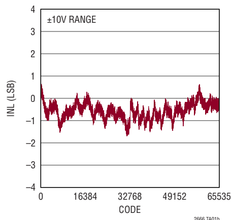
Integral Nonlinearity (LTC2666-16)
