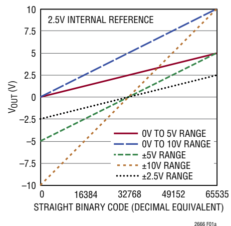
2a. LTC2666-16 Transfer Function
